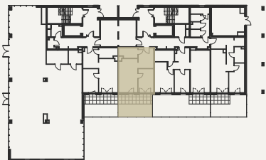
SCHEMAT PARTERU
